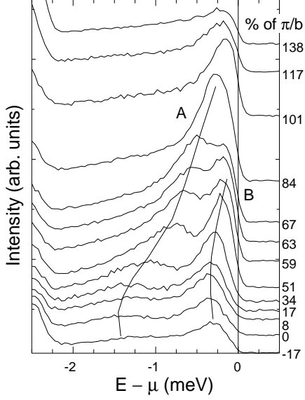
Figure 15: ARPES data of K_{0.3}MoO_3 taken at h\nu = 20 eV, \Delta E = 100 meV, \Delta\theta = \pm 1^\circ and T = 220 K. Thin lines are guides to the eye for dispersions.
